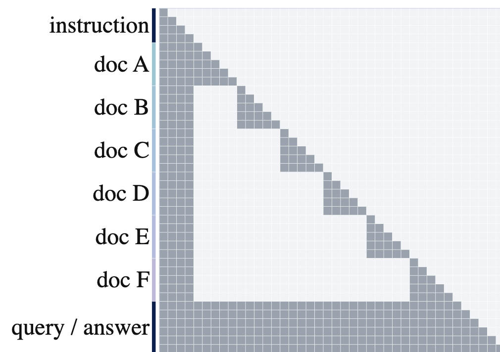
Document-chunked
