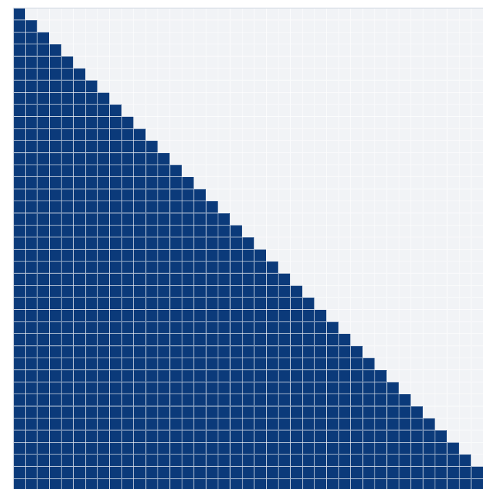
Full causal
